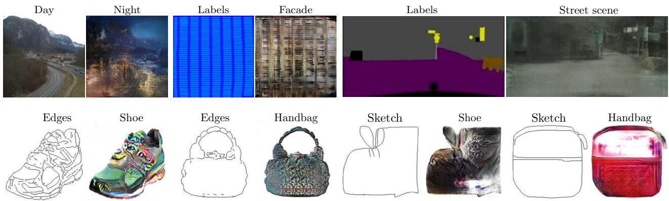
Figure 17: Example failure cases. Each pair of images shows input on the left and output on the right. These examples are selected as some of the worst results on our tasks. Common failures include artifacts in regions where the input image is sparse, and difficulty in handling unusual inputs. Please see https://phillipi.github.io/pix2pix/ for more comprehensive results.
