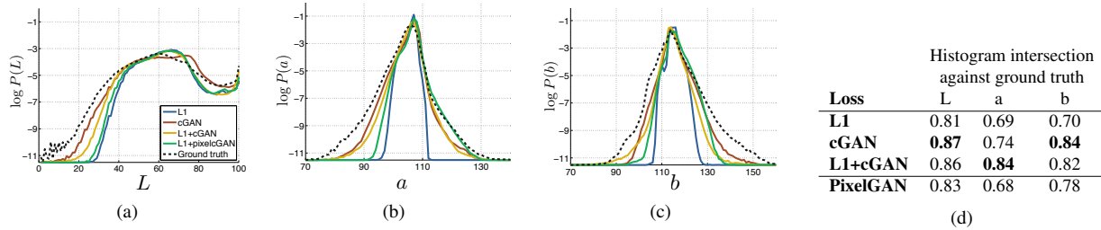
Figure 7: Color distribution matching property of the cGAN, tested on Cityscapes. (c.f. Figure 1 of the original GAN paper [14]). Note that the histogram intersection scores are dominated by differences in the high probability region, which are imperceptible in the plots, which show log probability and therefore emphasize differences in the low probability regions.
